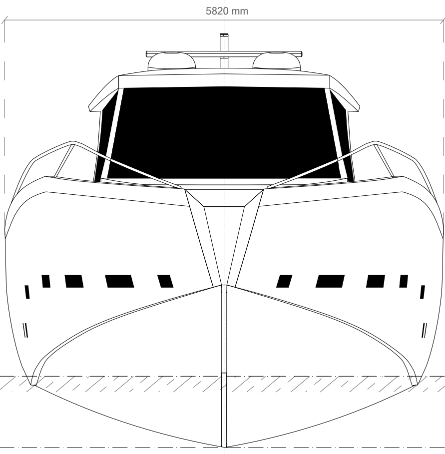
RIGHT VIEW
