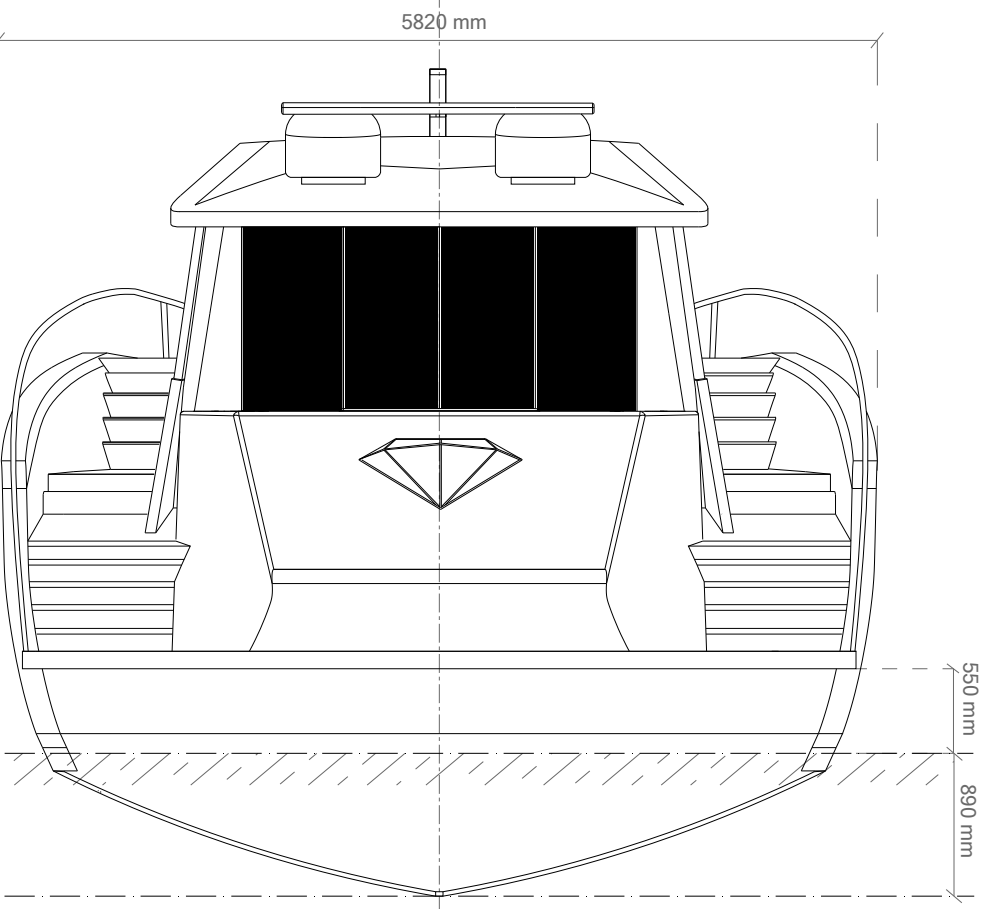
LEFT VIEW
